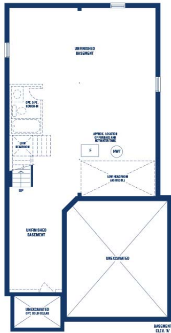
BASEMENT ELEV. 'A'
